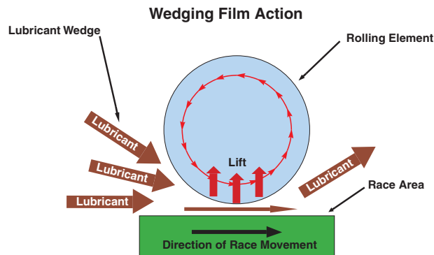
Full Fluid Film (Hydrodynamic) Condition
