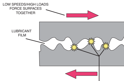
Lubricant film is too thin to provide total surface separation. Contact between surface asperities (or microscopic peaks and valleys) occurs. Friction reduction and wear protection is then only provided through chemical additives.
